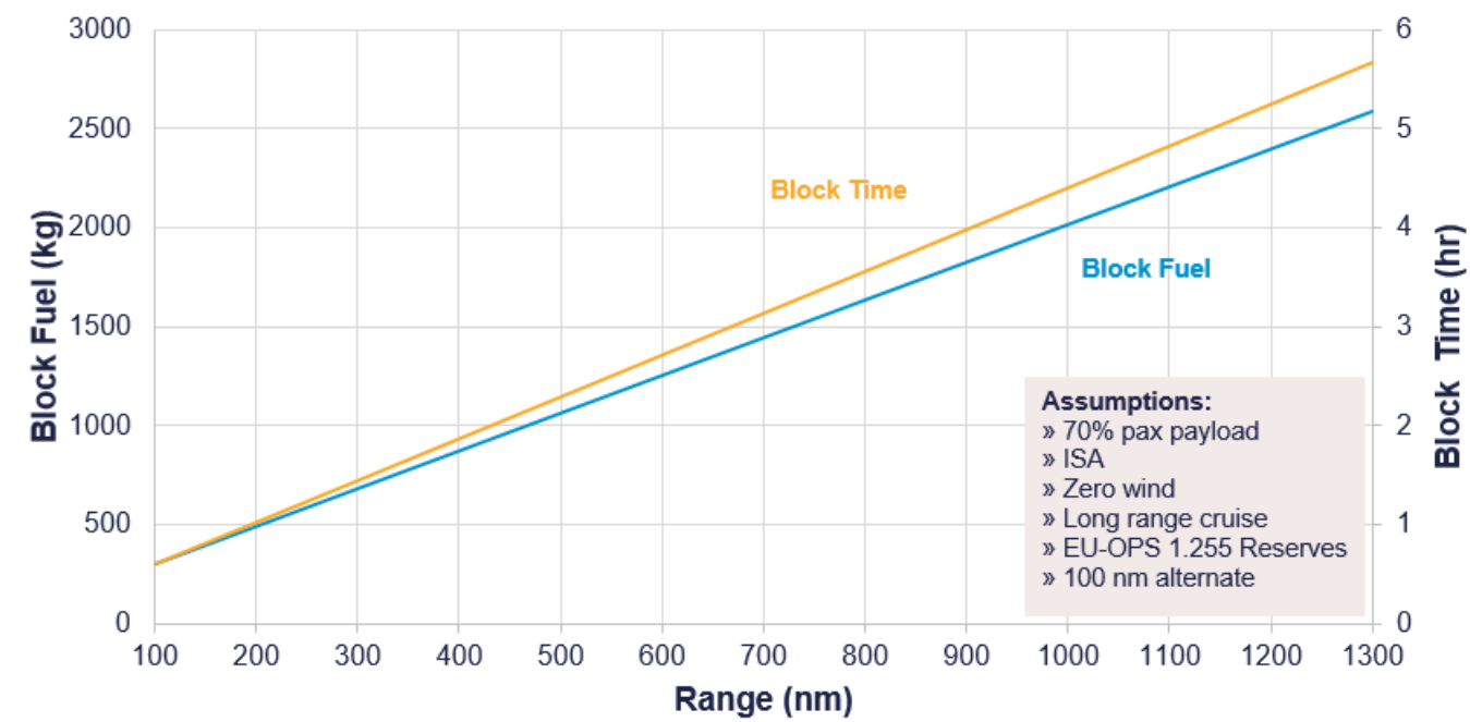
Fokker 50 - BF & BT vs Range
