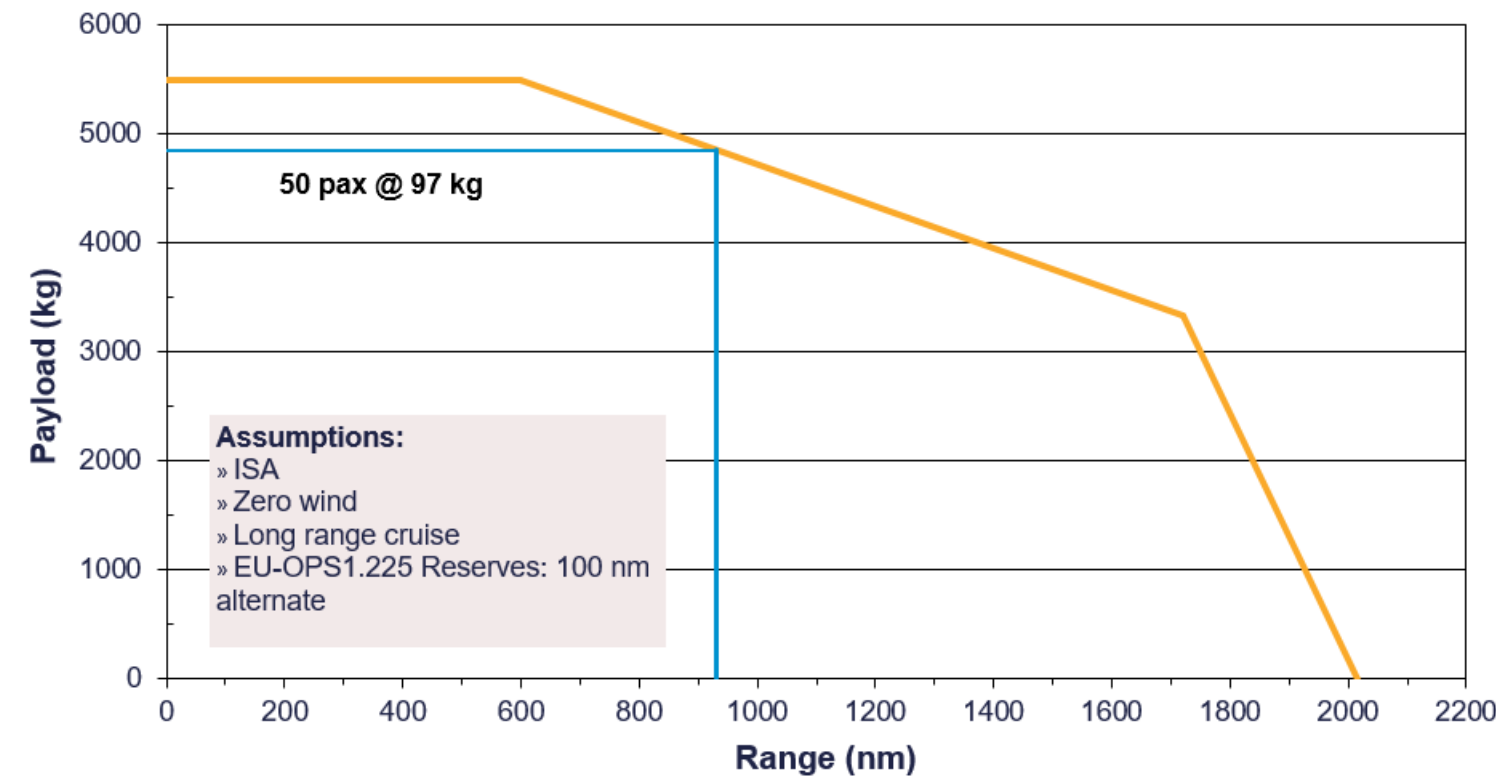
Payload vs Range
